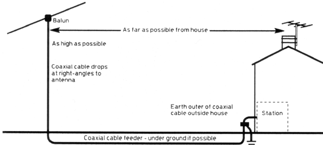
Fig 1 An antenna Installation with EMC in Mind
