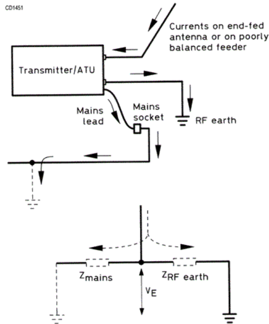
Fig 2 Earth current divides between RF earth and the mains. The current down each path will depend on the impedances. The earth terminal will be at V_E relative to "true" earth
